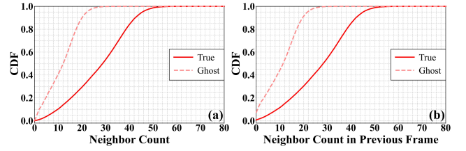
Figure 8: (a) CDF of a point's neighbor counts within a radius of 0.8m; (b) CDF of a point's neighbor counts within a radius of 0.8m in the previous frame.
