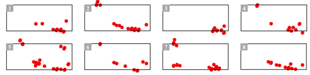
Figure 4: Radar points from an occluded vehicle in 8 consecutive frames (30 FPS), in which the black boxes represent the vehicle’s bounding boxes.
