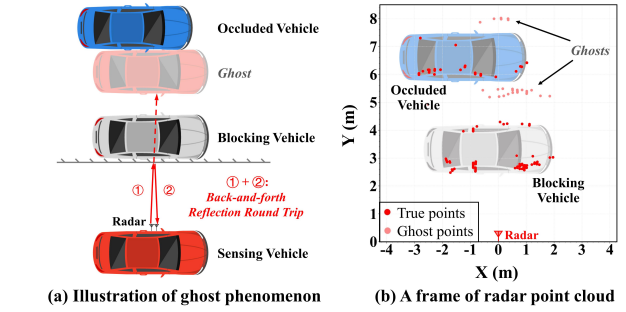
Figure 3: (a) Signals bounce between the vehicles, creating “ghost” vehicles. (b) Ghost points appear around true points from the occluded vehicle.
