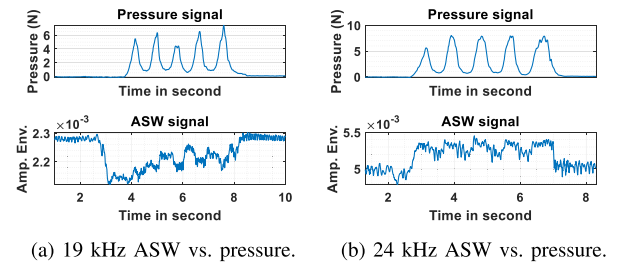
Fig. 8. The ASW signal responds to the touch force differently for different frequencies. The 24 kHz ASW signal in this example projects the pressure better than the 19 kHz ASW signal.
