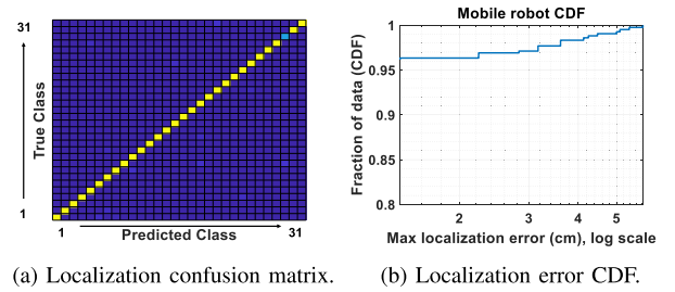
Fig. 14. The localization (a) confusion matrix and (b) error CDF in SonicSkin for mobile robot. We collected 16492 real-world datapoints in this experiment.
