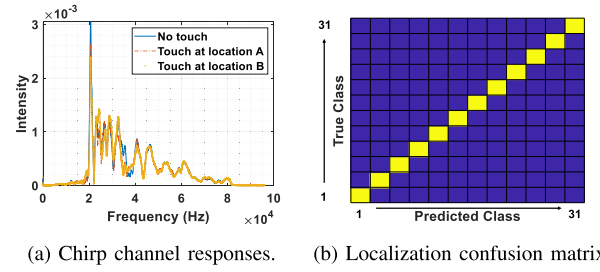
Fig. 4. We employ the chirp channel response differences \Delta H(f) caused by touches to localize the contact. (a) The chirp channel responds differently when there is no touch, touch at location A, and touch at location B (2 cm away from location A). (b) SonicSkin can accurately localize every touch in all locations that surround the robot arm in a proof-of-concept experiment.
