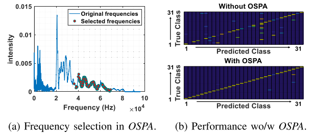
Fig. 6. OSPA selects frequencies that are sensitive to the touch but insensitive to the robot movement. (a) The selected frequencies from OSPA are mostly from 40 kHz to 70 kHz. (b) An example experimental result. The top and bottom confusion matrix shows the localization performance without and with OSPA , respectively. OSPA greatly improves the localization accuracy for mobile robot.
