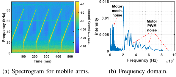
Fig. 5. The Spectrogram \mathcal{R}(t, f) and frequency domain R(f) of received ASW chirp when the robot is moving. The major mechanical noise resides in the lower frequency while there are three distinct noise peaks from the motor PWM at 30 kHz, 60 kHz, and 90 kHz.
