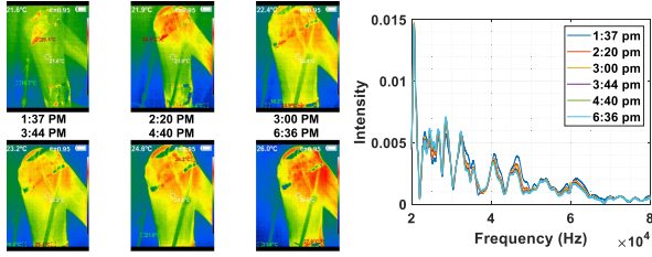
(a) Heat images of the Jaco arm. (b) Frequency response vs time.
